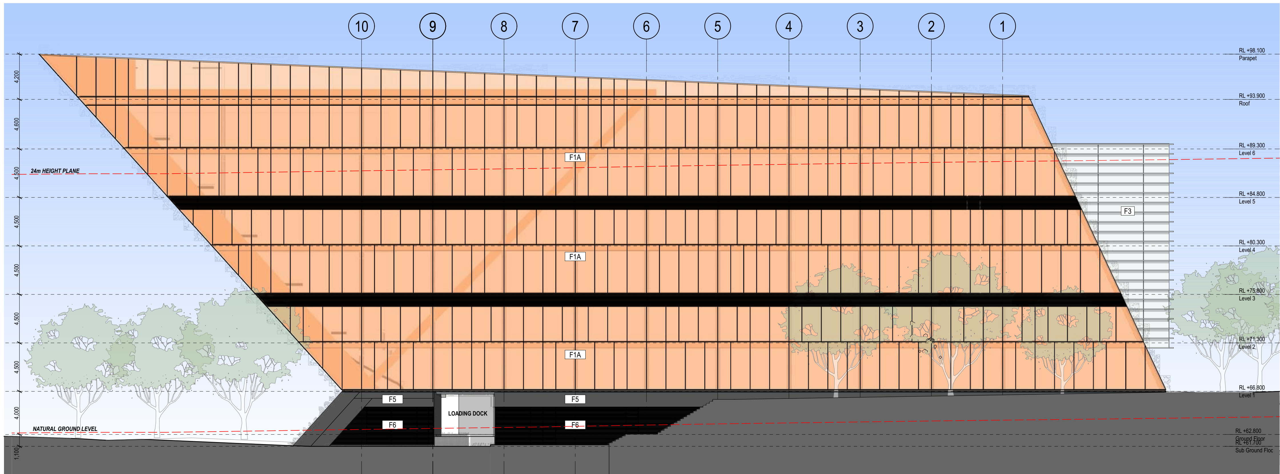
4 ELEVATION West 1:200
