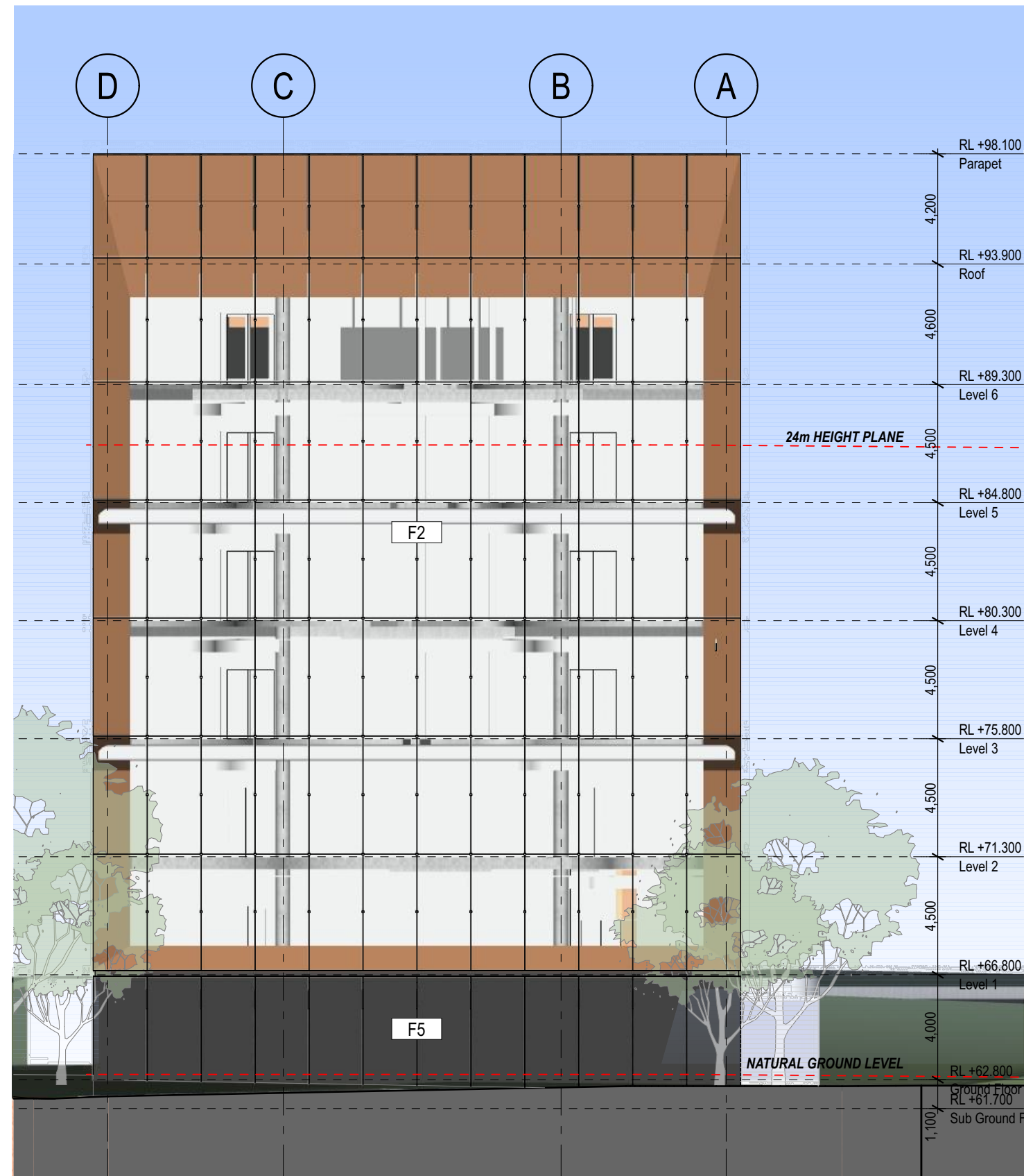
1 ELEVATION North 1:200
