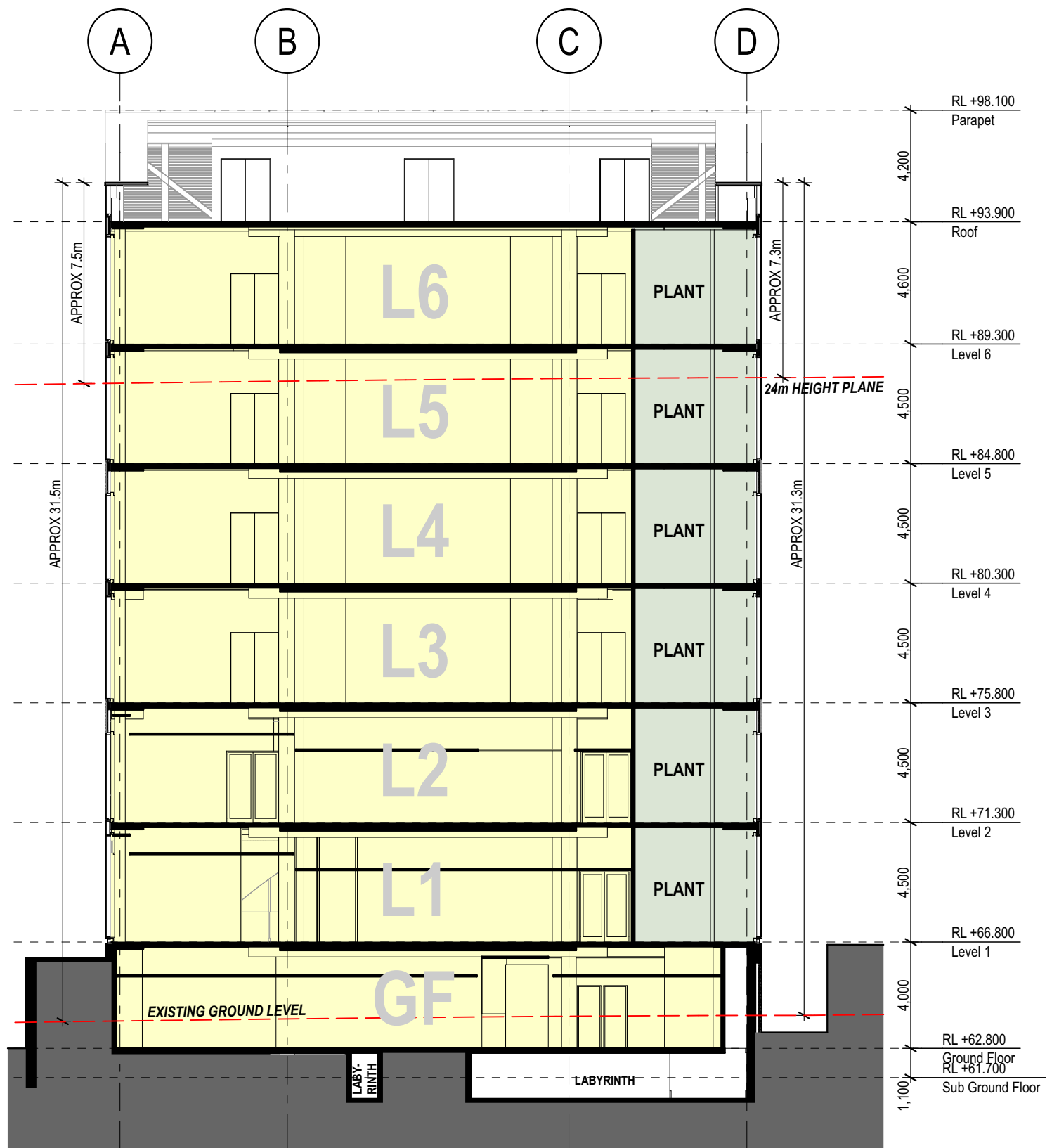
4 SECTION Section B2 1:200
