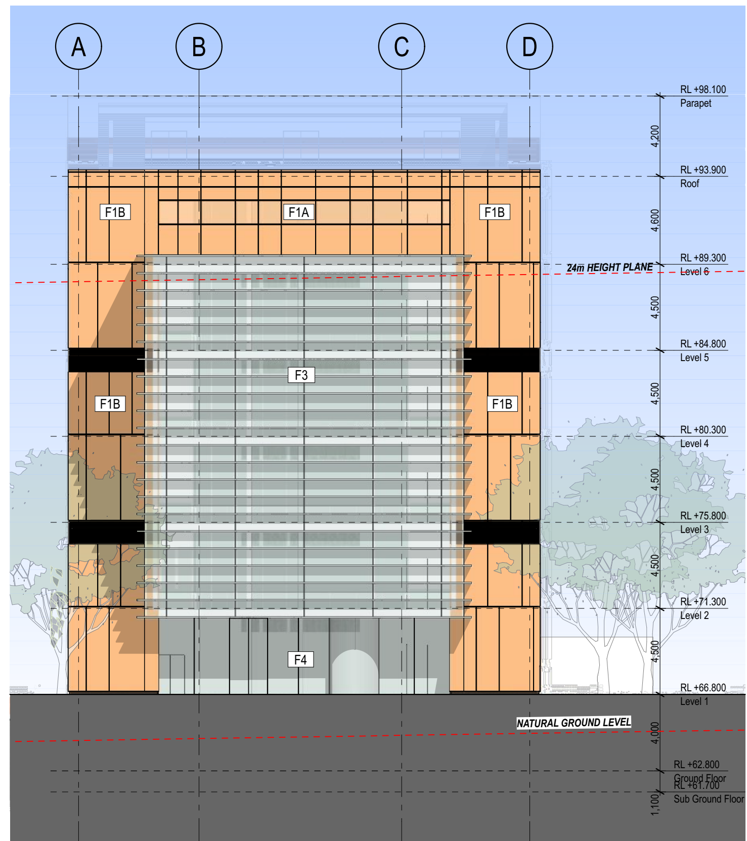
3 ELEVATION South 1:200
