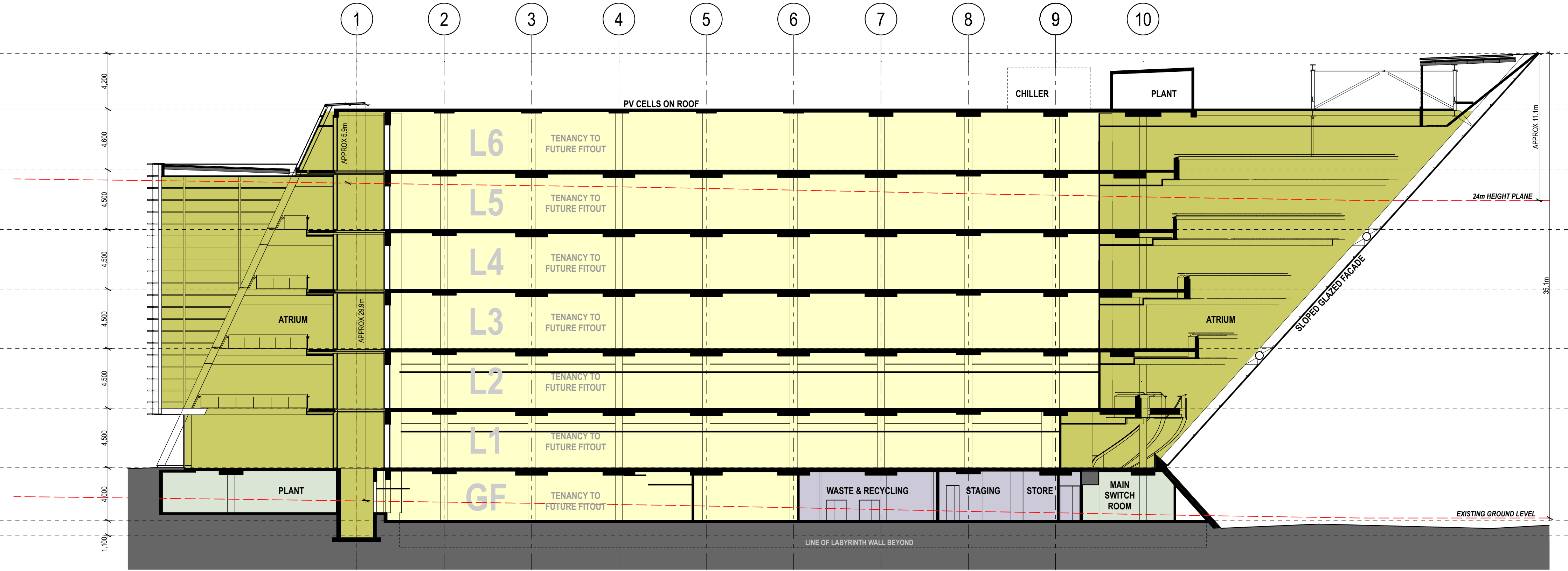
1 SECTION Section A1 1:200
