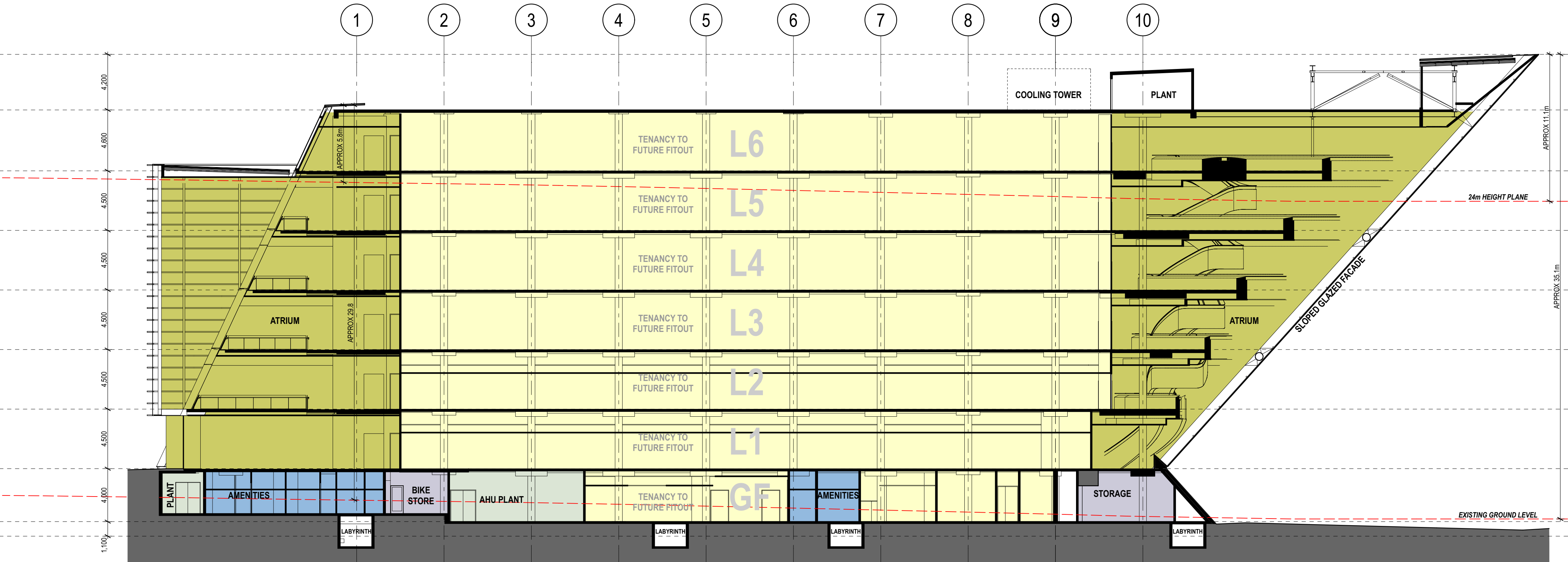
3 PLAN Section A2 1:200
