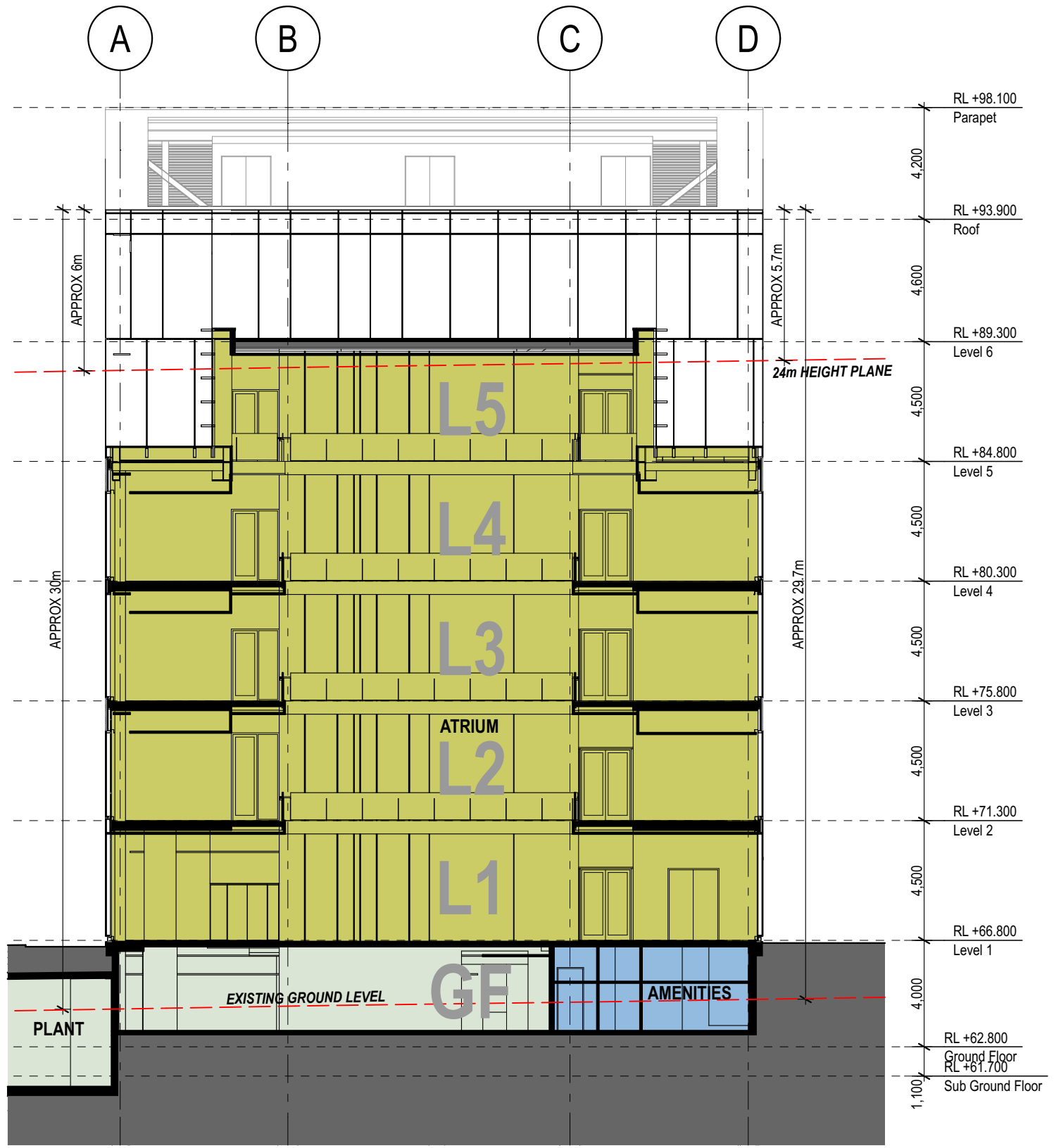
2 SECTION Section B1 1:200
