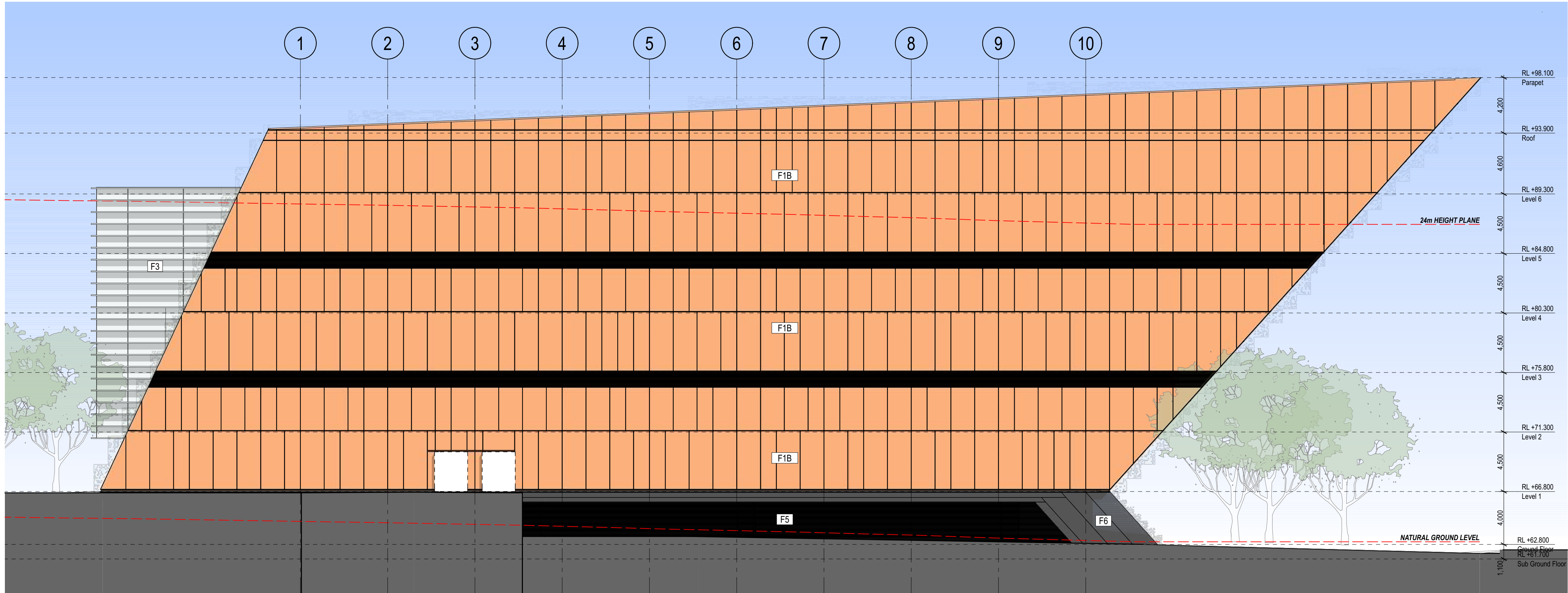
2 ELEVATION East 1:200
